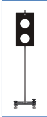
15. X-431 ADAS Nissan AVM target configuration(LAC04-15)
